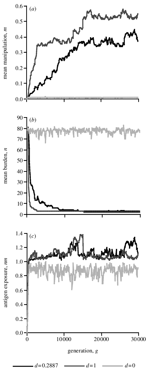
Figure 1. Representative invasion dynamics of adaptive CI under three separate conditions of density dependence ( d = 0 , d = 0.2887 and d = 1 ). (a) The mean adaptive adult-derived larval antigen m , (b) the mean chronic worm burden n , and (c) the mean host exposure to larval antigen nm as a function of the generation number g . \lambda = 80 , T = 0.5 , c = 0.01 , v = 1 , a = l = 0 , host number = 100 and mutation rate = mutation distance = 0.01.
